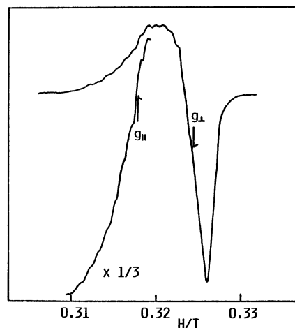
Fig. 7. ESR spectrum of the electrochemically oxidized form of the oxygenated complex 1 ( [\text{Co}_2(\text{tpdp})(\text{CH}_3\text{COO})(\text{O}_2)]^{2+} ) in acetonitrile at liquid \text{N}_2 temperature.
