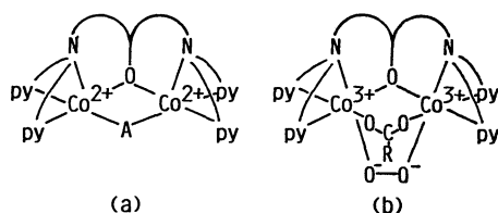
Fig. 3. Possible structures of dinuclear cobalt complexes.
