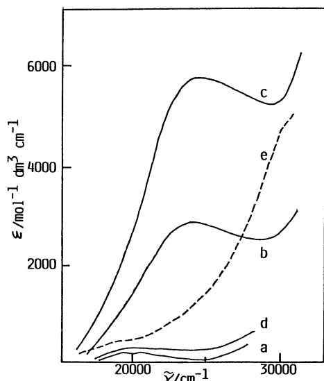
Fig. 5. Spectral change of 2 ( [\text{Co}_2(\text{tmdp})(\text{CH}_3\text{COO})]^{2+} ) at various oxygen pressures in dichloromethane at 20°C. The spectra of a–c are at the partial oxygen pressures: 0, 3, 700 Torr, respectively. The spectrum d is at 0 Torr after one oxygenation-deoxygenation cycle. The spectrum e is the one measured under the air after standing the oxygenated solution for 4 days (----).
