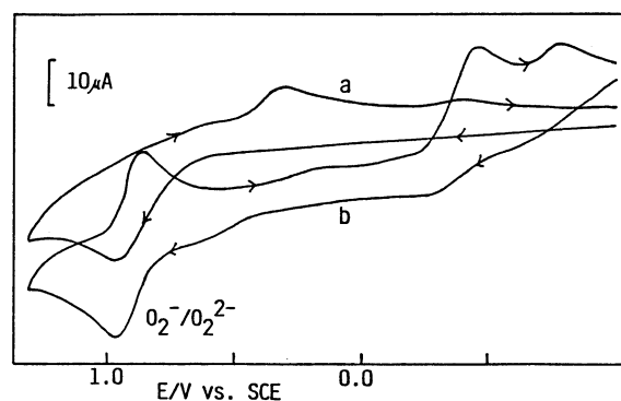
Fig. 6. Cyclic voltammograms of 3 ( [\text{Co}_2(\text{bpm})-(\text{CH}_3\text{COO})]^{2+} ) (a) and 3a ( [\text{Co}_2(\text{bpm})(\text{CH}_3\text{COO})(\text{O}_2)]^{2+} ) (b) in acetonitrile ( 0.1 \text{ mol dm}^{-3} tetrabutylammonium perchlorate) at a glassy carbon electrode at scan rate of 100 \text{ mV s}^{-1} .
