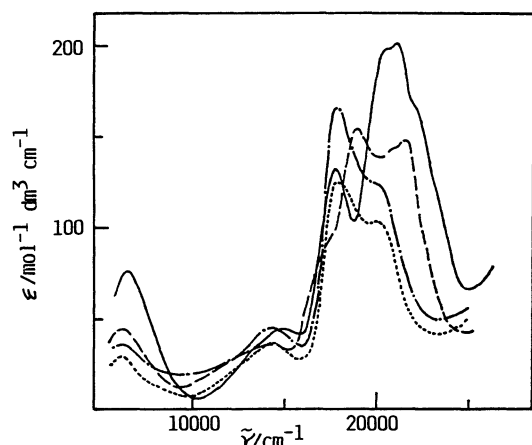
Fig. 2. Electronic spectra of 1 ( [\text{Co}_2(\text{tpdp})(\text{CH}_3\text{COO})]^{2+} ) (—), 2 ( [\text{Co}_2(\text{tmdp})(\text{CH}_3\text{COO})]^{2+} ) (---), 4 ( [\text{Co}_2(\text{tmdp})\text{Cl}]^{2+} ) (.....), and 5 ( [\text{Co}_2(\text{tmdp})\text{Br}]^{2+} ) (— · —) in acetonitrile.
