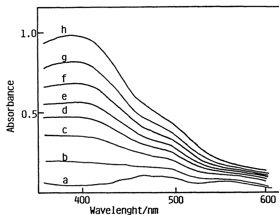
Fig. 4. Spectral change of 1 ( [\text{Co}_2(\text{tpdp})(\text{CH}_3\text{COO})]^{2+} ) at various oxygen pressures in acetonitrile at -15.2^\circ\text{C} . Spectra of a—h are at the partial oxygen pressures: 0, 68, 149, 213, 280, 373, 497, and 756 Torr, respectively.
